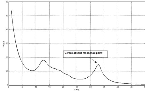
Fig. 2. Conductance curve
