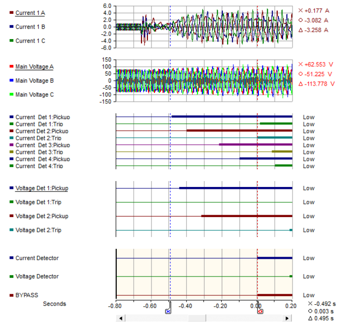
Fig. 9. Oscillography captured by the relay
