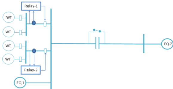
Fig. 7. Windfarm tripping
