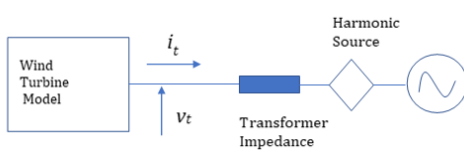
Fig. 3. Dynamic frequency scan setup
