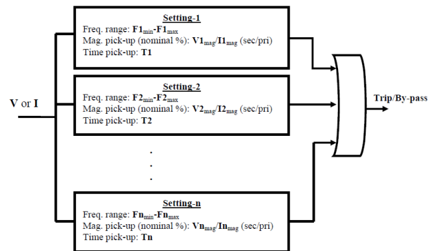
Fig. 8. Generic protection logic
